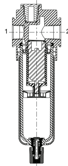
Cross Section - 651/652/653 Series Particulate Filter
