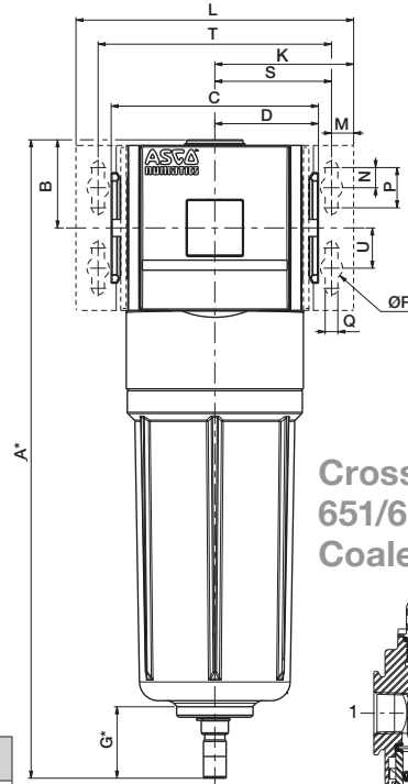
653 Series High Flow
