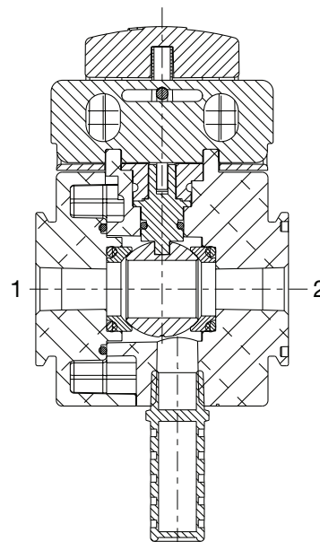
Cross Section - 651/652/653 Series Shut Off Isolation Valve
