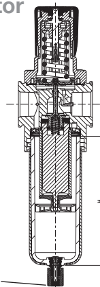
Cross Section - 651/652/653 Series Particulate Filter/ Regulator
